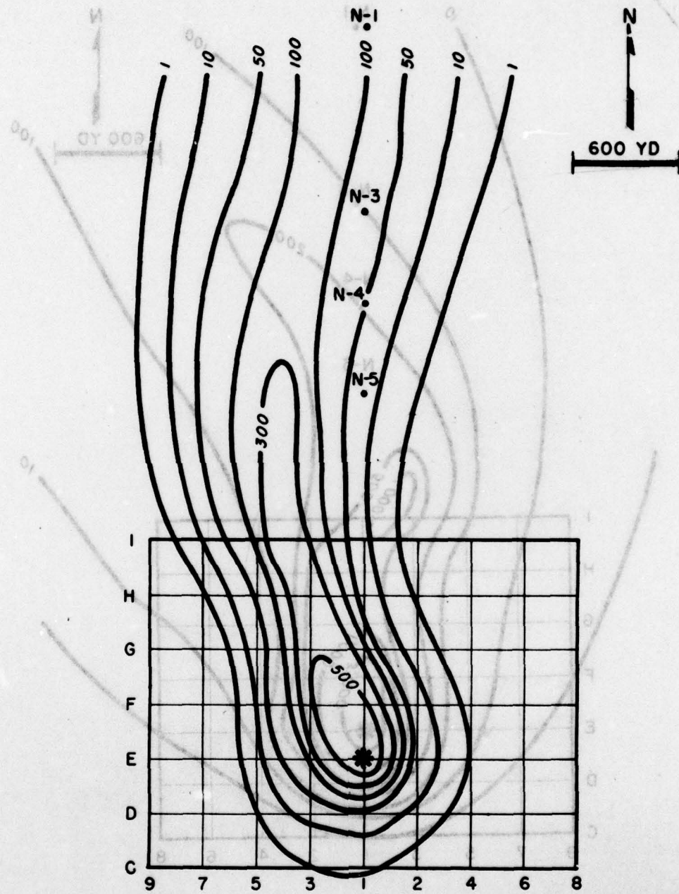
Fig. A.9 Surface Explosion Field Gamma, as Roentgens per Hour one Hour after Burst, for Project 2.5a-2, (Fig. 4.19, WT-371). Intersections of Grid Lines Represent Station Locations.
